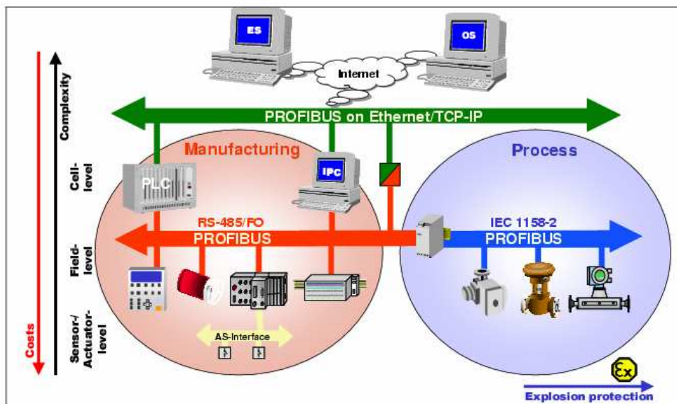
Fig. 1: Industrial Communication
