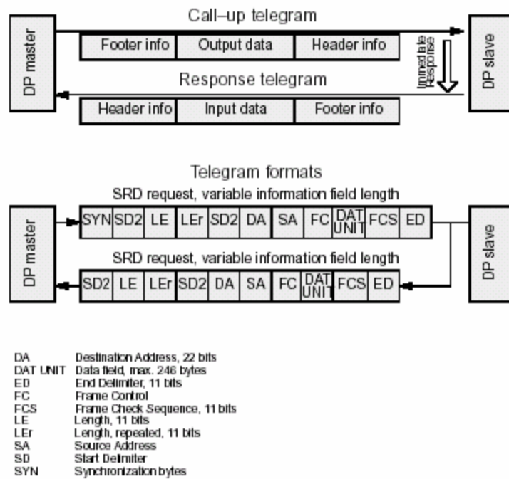
Figure 7 User Data Transmission Principle
