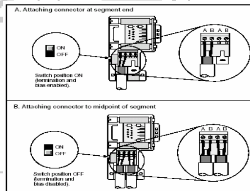
Figure 3-10 Attaching Connector and Selecting Termination
