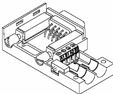
Figure 1-1. Seimens Bus Connector
