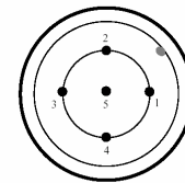
M12 Connector for RS-485 in IP65/67 Pin assignment: 1: VP, 2: RxD/TxD-N 3: DGND, 4: RxD/TxD-P, 5: Shield
